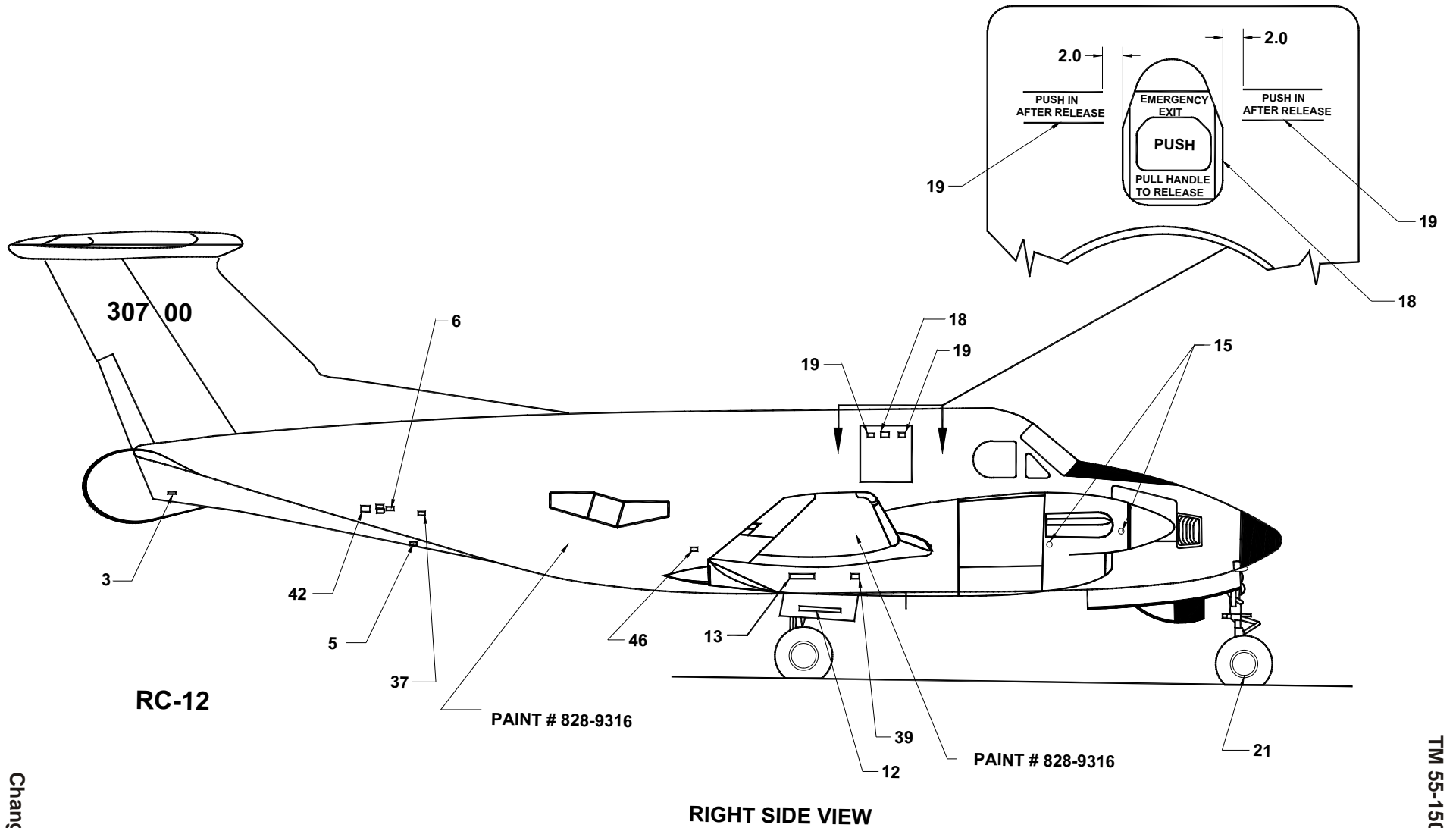
Figure 10-1. Exterior Markings, RC-12 (Sheet 6 of 22)
