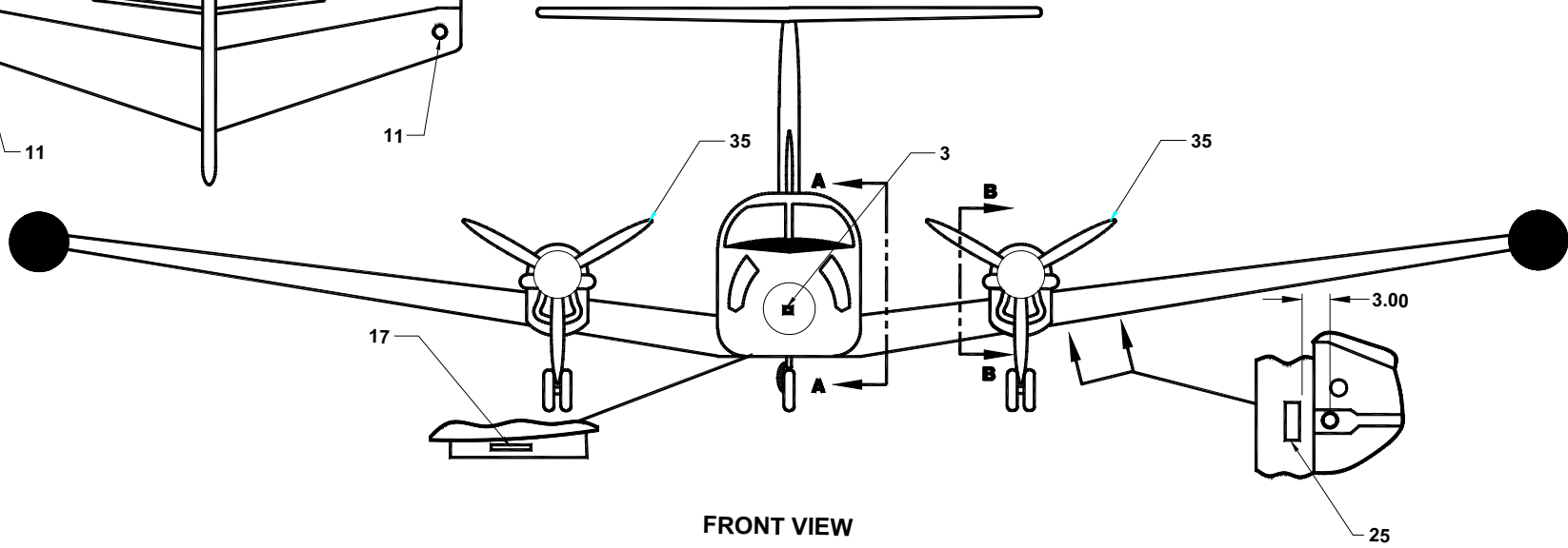
Figure 10-1. Exterior Markings, RC-12 (Sheet 10 of 22)
