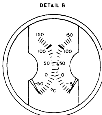
OIL TEMPERATURE GAGE
