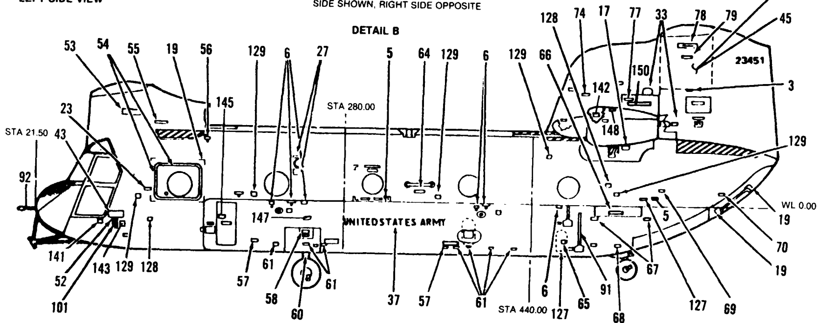
Figure 9-10. Exterior Markings, CH-47 (Sheet 2 of 29)
